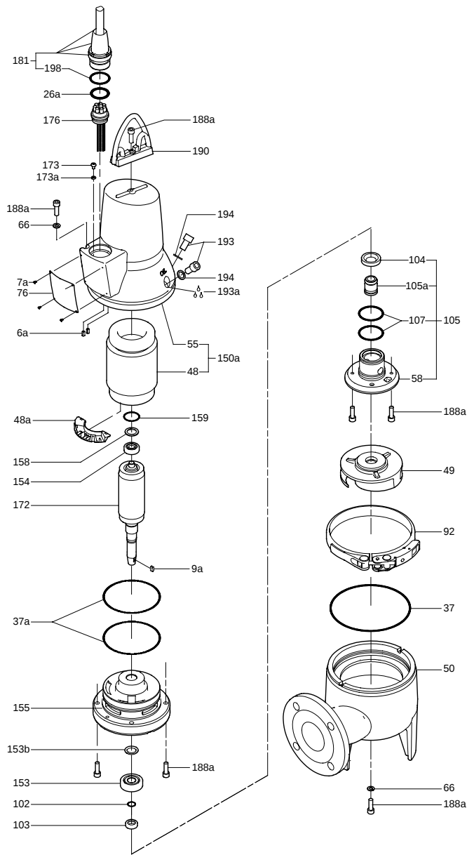
Fig. D Exploded view of SEV.65 pump
