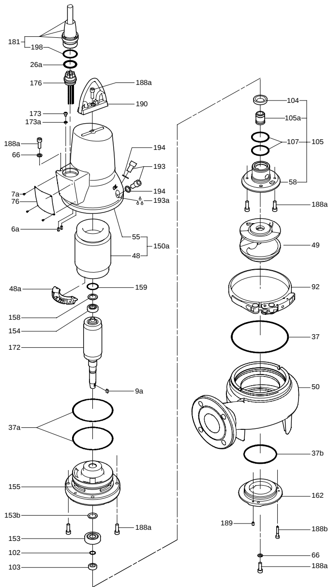
Fig. C Exploded view of SE1.50 pump
